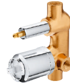
DV-1002 46 MM High Flow Single Lever Diverter Exposed Part Kit For Operating Lever, Wall Flange & Button M.R.P. : 4790/-
